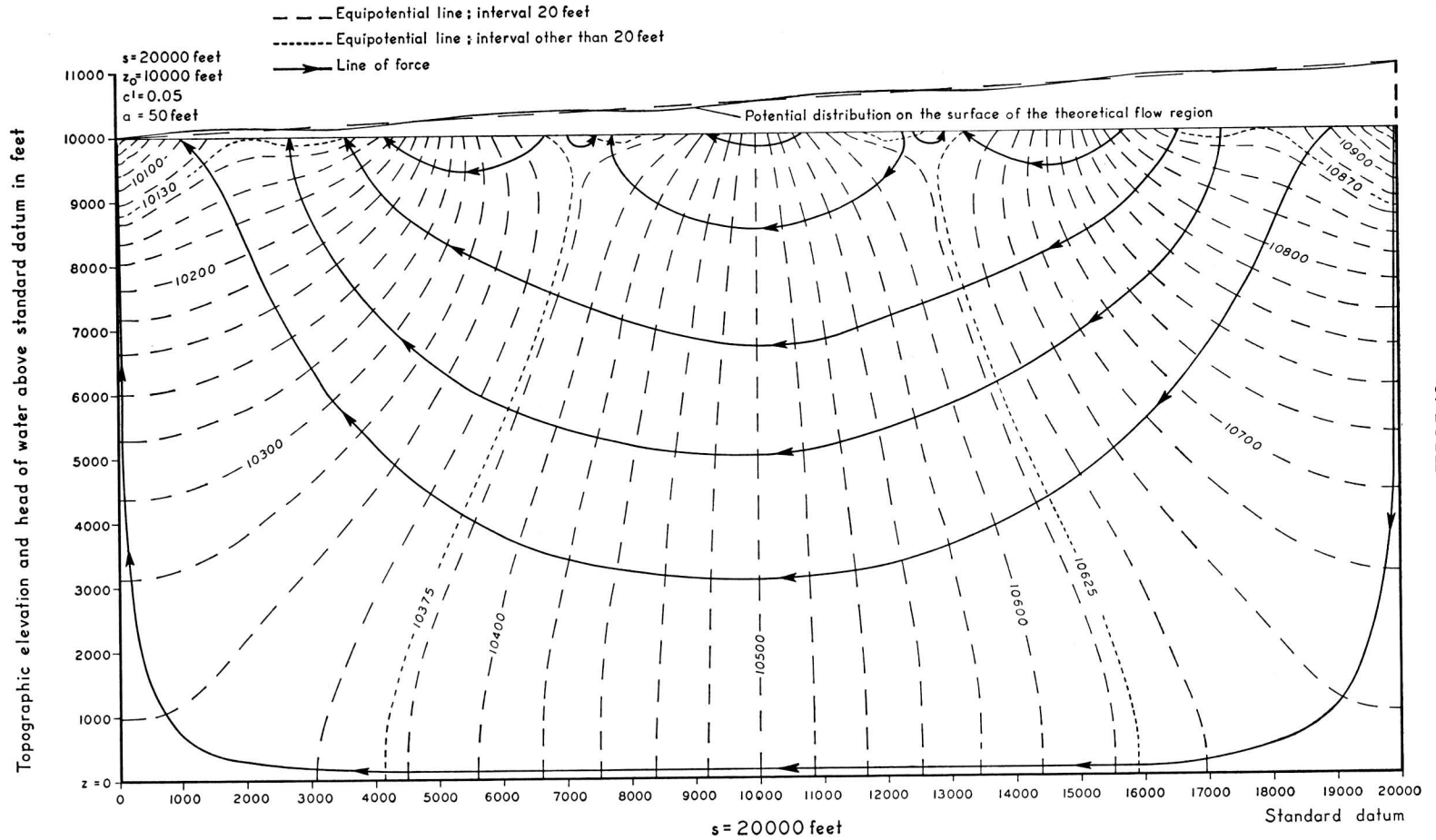
Fig. 2 h . Potential distribution and flow pattern as obtained by equation 6.
